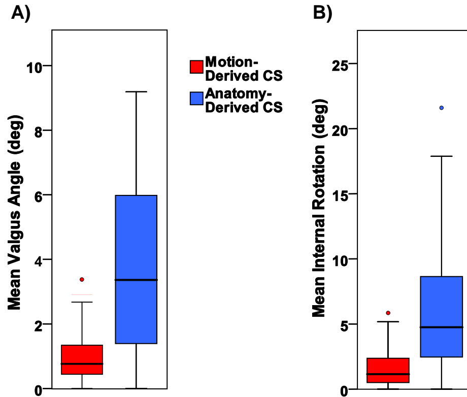
Figure 4.4: Inter-Subject Variability
